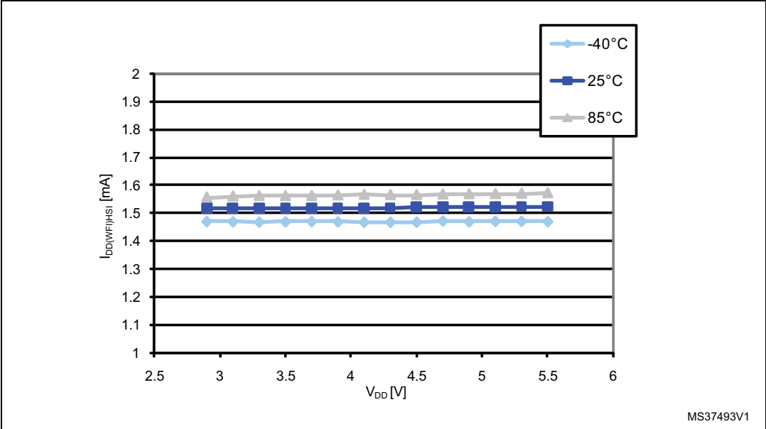
Figure 16. Typ. I_{DD(WFI)} vs V_{DD} , HSI RC osc, f_{CPU} = 16\text{ MHz}
