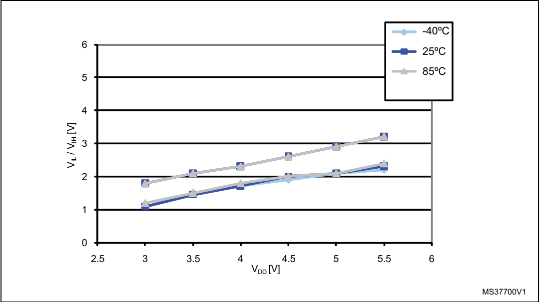
Figure 21. Typical V_{IL} and V_{IH} vs V_{DD} @ 3 temperatures
