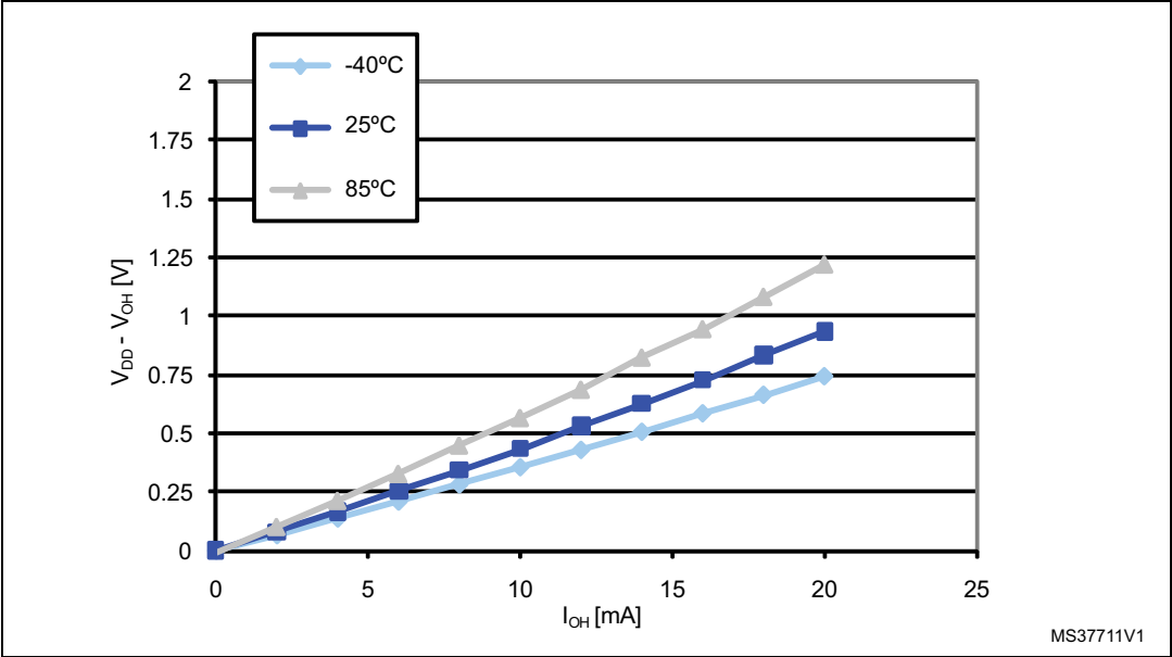
Figure 32. Typ. V_{DD} - V_{OH} @ V_{DD} = 5\text{ V} (high sink ports)
