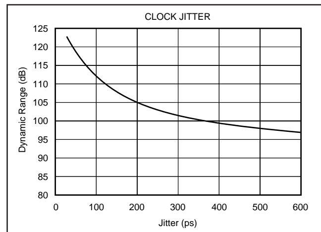
FIGURE 21. Jitter Sensitivity.
