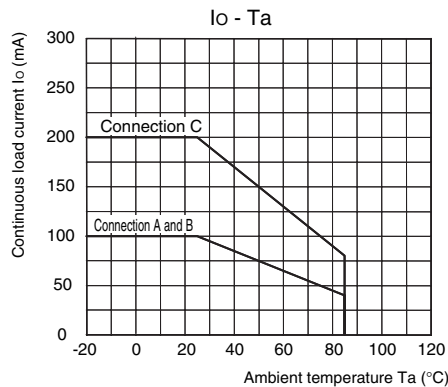
Continuous load current vs. Ambient temperature
