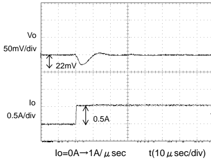
Fig.2 Transient Response (0→0.5A) Co=47 µ F, Cfb=1000pF
