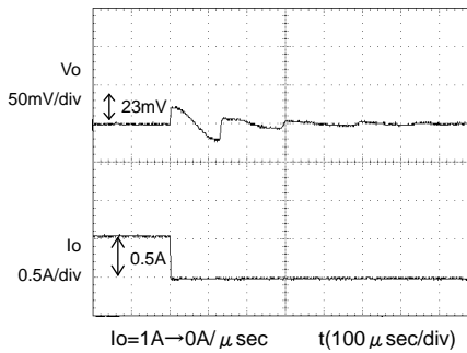
Fig.5 Transient Response (0.5→0A) Co=47 µ F, Cfb=1000pF
