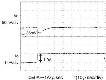
Fig.7 Transient Response (0→1.0A) Co=100 µ F, Cfb=1000pF
