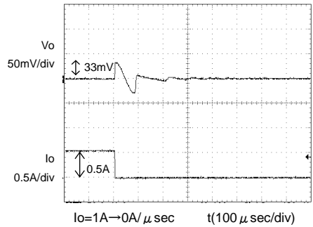
Fig.6 Transient Response (0.5→0A) Co=22 µ F, Cfb=1000pF
