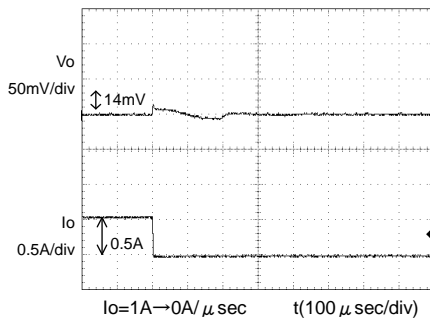
Fig.4 Transient Response (0.5→0A) Co=100 µ F, Cfb=1000pF
