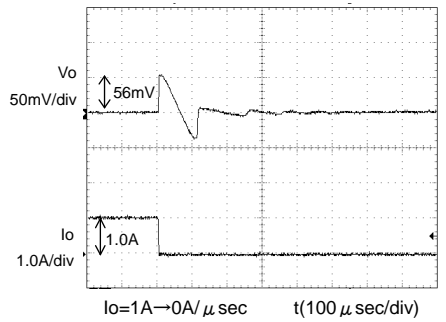
Fig.12 Transient Response (1.0→0A) Co=22 µ F, Cfb=1000pF
