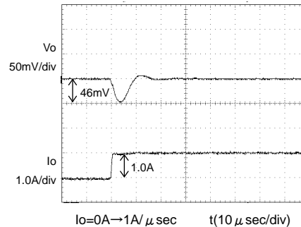
Fig.8 Transient Response (0→1.0A) Co=47 µ F, Cfb=1000pF
