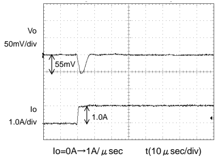
Fig.9 Transient Response (0→1.0A) Co=22 µ F, Cfb=1000pF
