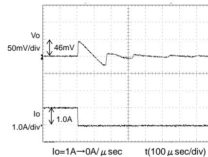
Fig.11 Transient Response (1.0→0A) Co=47 µ F, Cfb=1000pF
