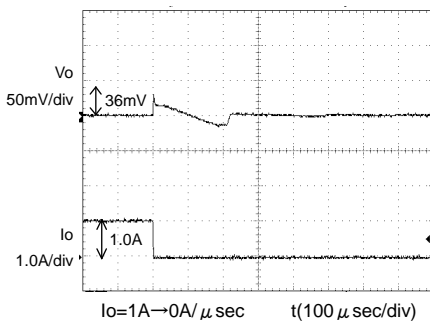
Fig.10 Transient Response (1.0→0A) Co=100 µ F, Cfb=1000pF
