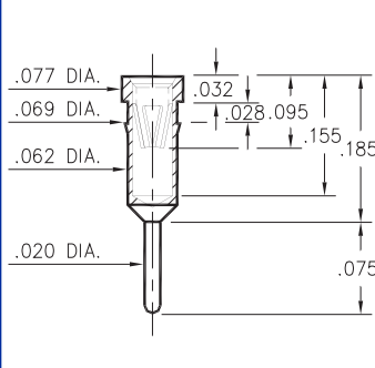
2400-0-15-XX-47-XX-04-0 Press-fit in .066 mounting hole.
