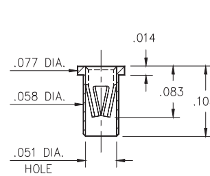
7305-0-15-XX-47-XX-10-0 Solder mount in .060 min. mounting hole Also available on 8mm wide carrier tape: 6,000 parts per 13" reel. Order as: 7305-0-57-XX-47-XX-10-0
