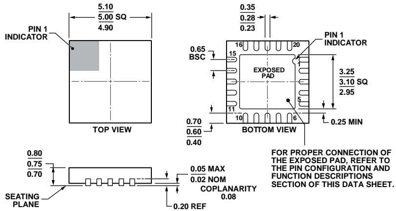
Figure 53. 20-Lead Lead Frame Chip Scale Package [LFCSP_WQ] 5 mm × 5 mm Body, Very Very Thin Quad (CP-20-9) Dimensions shown in millimeters
