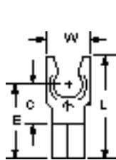
MU10-10FL 10 12-10
