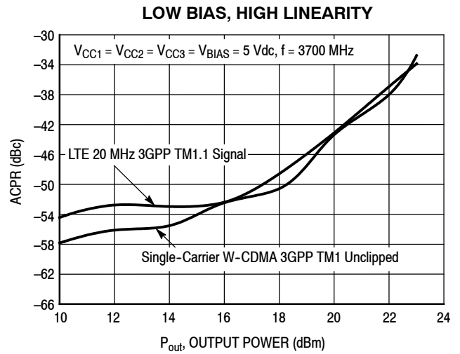
Figure 40. ACPR versus Output Power
