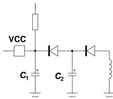
Figure 61. Split V_{CC} Supply
