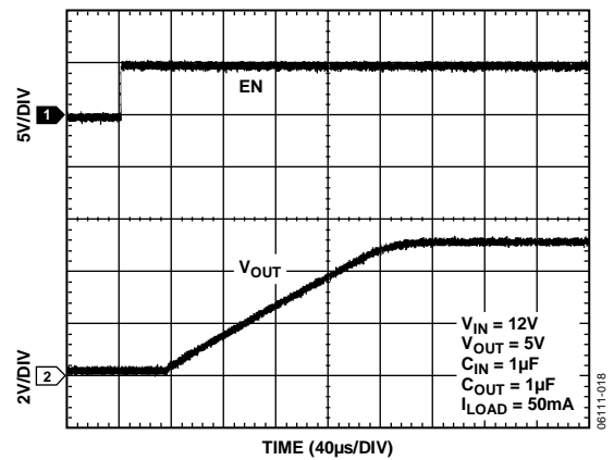
Figure 18. Start-Up Time
