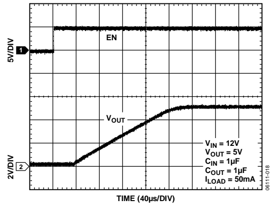
Figure 18. Start-Up Time
