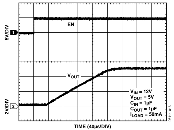
Figure 18. Start-Up Time
