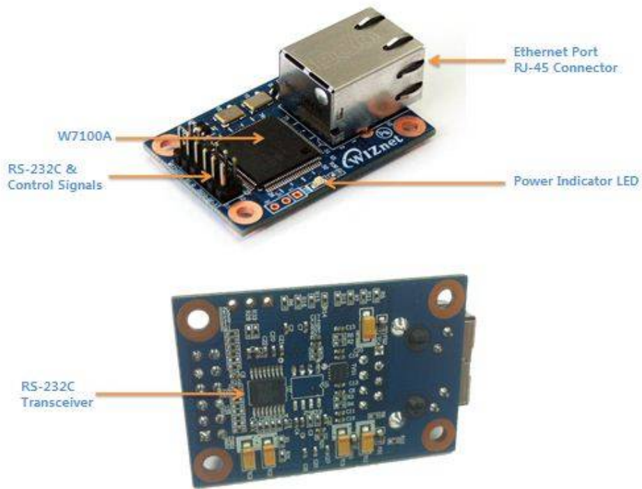
Figure 1. WIZ107SR Interface
