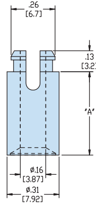
TWO PRONG SNAP LOCK / #6 SELF-TAPPING SCREW
