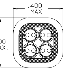
SECTION B-B STRAIN RELIEF CLAMP TJSS-106-6 AFTER CRIMPING SCALE 4:1
