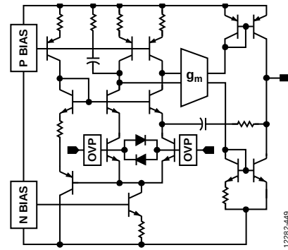
Figure 84. Conceptual Schematic
