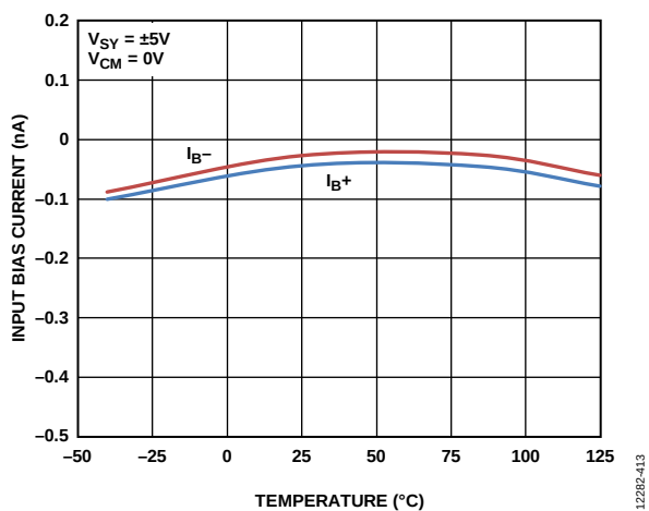
Figure 29. Input Bias Current ( I_B ) vs. Temperature, V_{SV} = \pm 5 V
