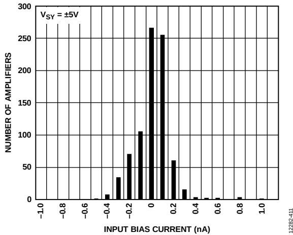
Figure 28. Input Bias Current Distribution, V_{SV} = \pm 5 V
