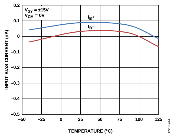
Figure 32. Input Bias Current ( I_B ) vs. Temperature, V_{SV} = \pm 15 V
