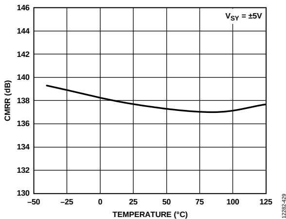
Figure 41. Common-Mode Rejection Ratio (CMRR) vs. Temperature, V_{SY} = \pm 5\text{ V}
