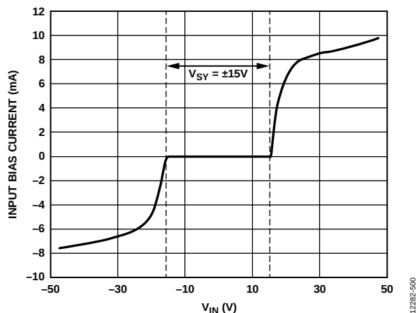
Figure 88. Input Bias Current During Positive and Negative Overvoltage, V_{SV} = \pm 15 V, Voltage Follower Configuration
