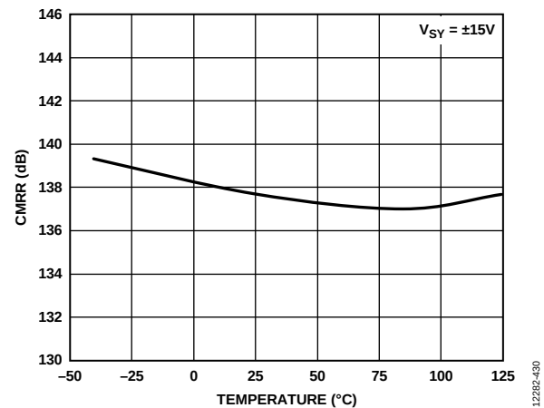
Figure 44. Common-Mode Rejection Ratio (CMRR) vs. Temperature, V_{SY} = \pm 15\text{ V}
