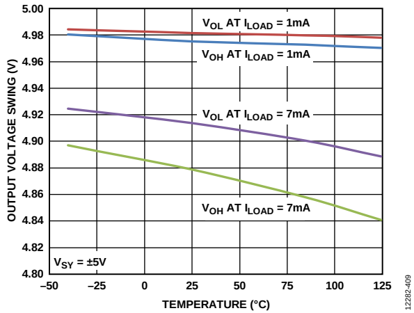
Figure 27. Output Voltage Swing vs. Temperature, V_{SV} = \pm 5 V
