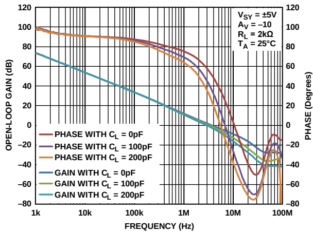
Figure 39. Open-Loop Gain and Phase vs. Frequency, V_{SY} = \pm 5\text{ V}
