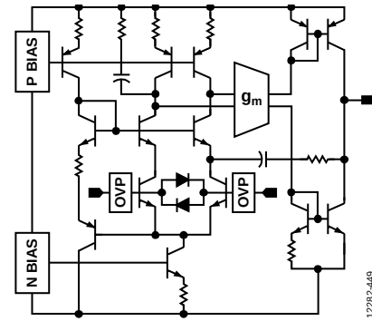
Figure 84. Conceptual Schematic
