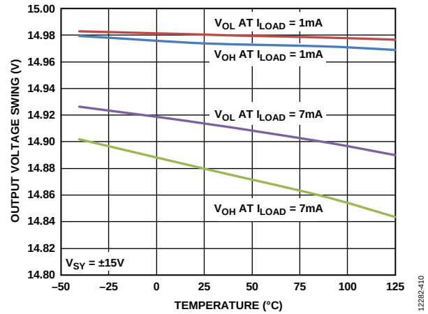
Figure 30. Output Voltage Swing vs. Temperature, V_{SV} = \pm 15 V
