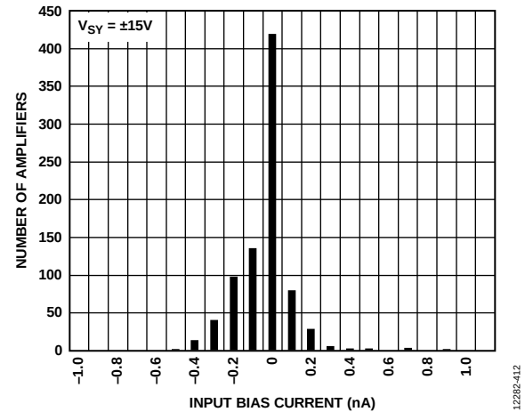
Figure 31. Input Bias Current Distribution, V_{SV} = \pm 15 V
