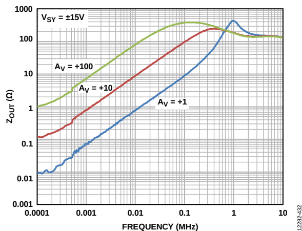
Figure 48. Output Impedance ( Z_{OUT} ) vs. Frequency, V_{SY} = \pm 15 V
