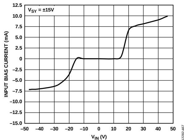
Figure 74. Input Bias Current vs. Input Voltage ( V_{IN} ) Including Input Overvoltage Range (Beyond V_{SY} = \pm 15V )
