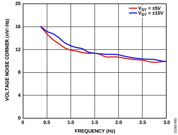
Figure 67. Voltage Noise Corner vs. Frequency, V_{SY} = \pm 5\text{ V} and V_{SY} = \pm 15\text{ V}
