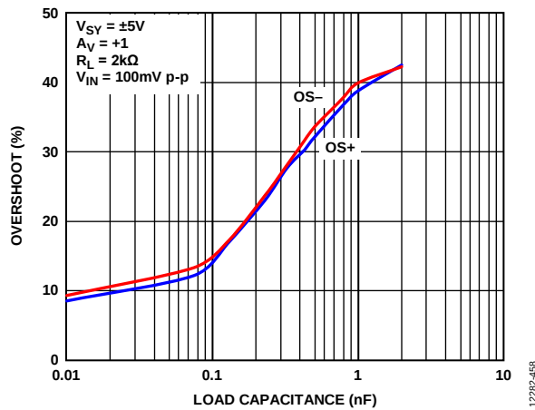
Figure 58. Small Signal Overshoot vs. Load Capacitance, V_{SV} = \pm 5\text{ V}
