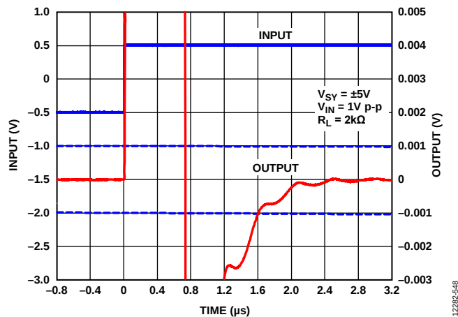
Figure 59. Positive Settling Time to 0.1%, V_{SV} = \pm 5\text{ V}
