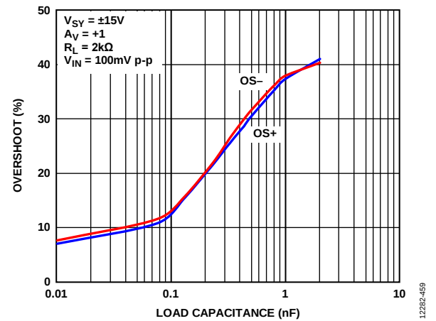
Figure 61. Small Signal Overshoot vs. Load Capacitance, V_{SV} = \pm 15\text{ V}
