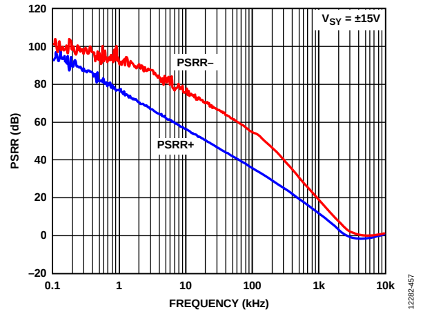
Figure 60. Power Supply Rejection Ratio (PSRR) vs. Frequency, V_{SV} = \pm 15\text{ V}
