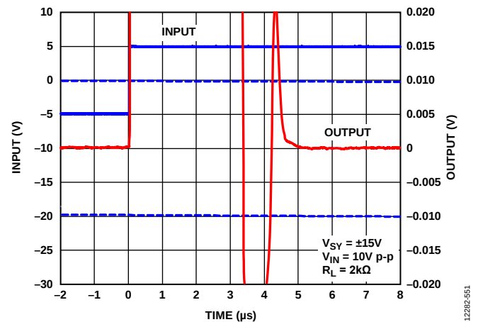
Figure 62. Positive Settling Time to 0.1%, V_{SV} = \pm 15\text{ V}
