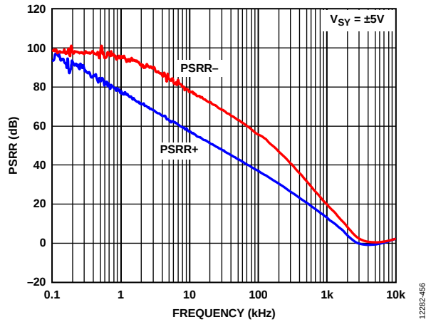
Figure 57. Power Supply Rejection Ratio (PSRR) vs. Frequency, V_{SV} = \pm 5\text{ V}
