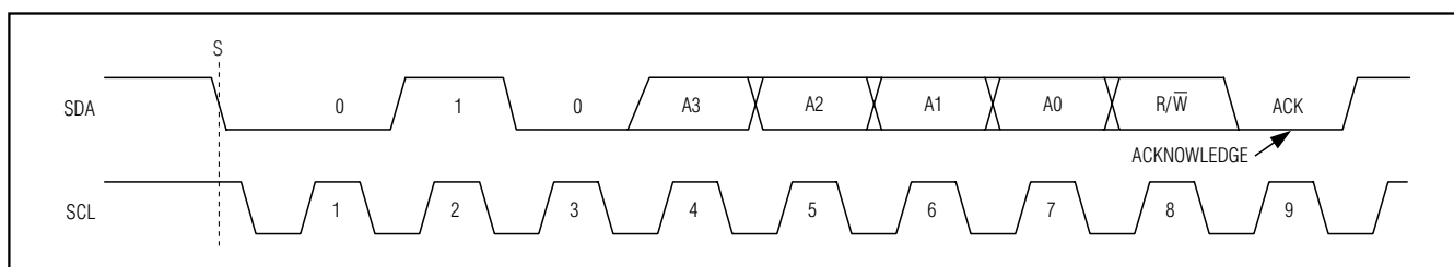
Figure 8. Slave Address Byte
