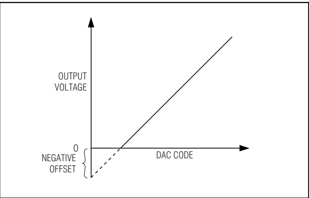
Figure 10. Effect of Negative Offset (Single Supply)
