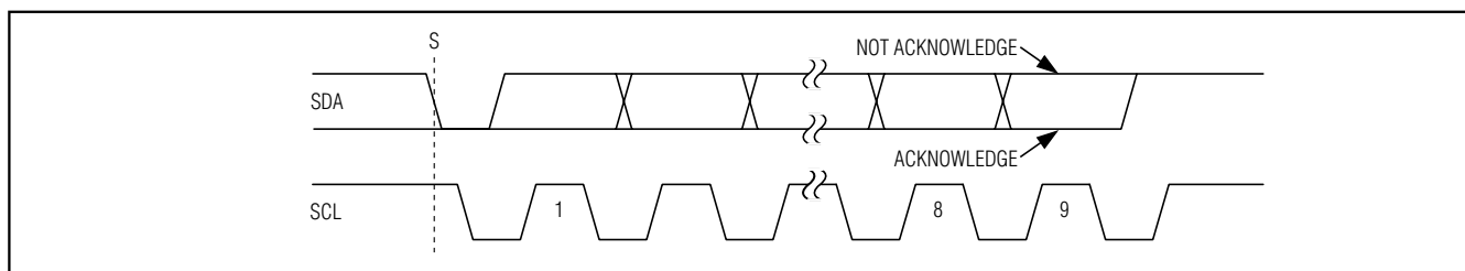
Figure 7. Acknowledge and Not-Acknowledge Bits
