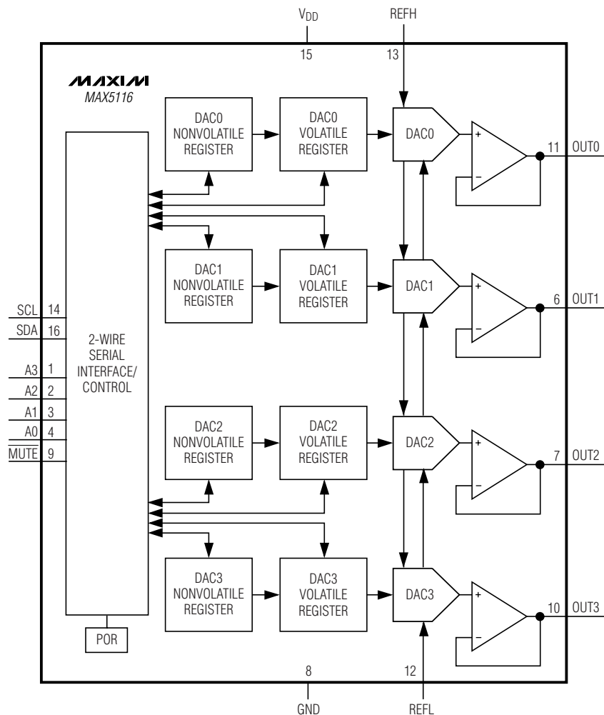
Figure 2. MAX5116 Functional Diagram
