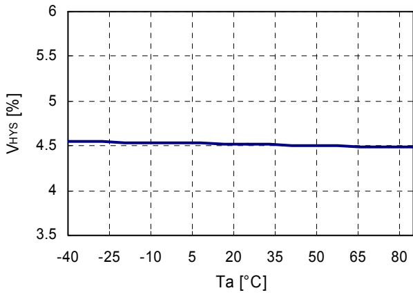
RP600KxxxA/B/D VIN=3.0V
