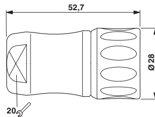
Dimensional drawing
