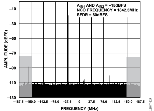
Figure 27. Two-Tone FFT; f_{IN1} = 1800 MHz, f_{IN2} = 2100 MHz f_{CLK} = 2.94912 GHz; Decimation Ratio = 8, NCO Frequency = 1874.28 MHz
