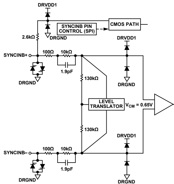
Figure 45. SYNCINB± Inputs
