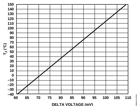
Figure 75. Junction Temperature vs. \Delta V (mV)
