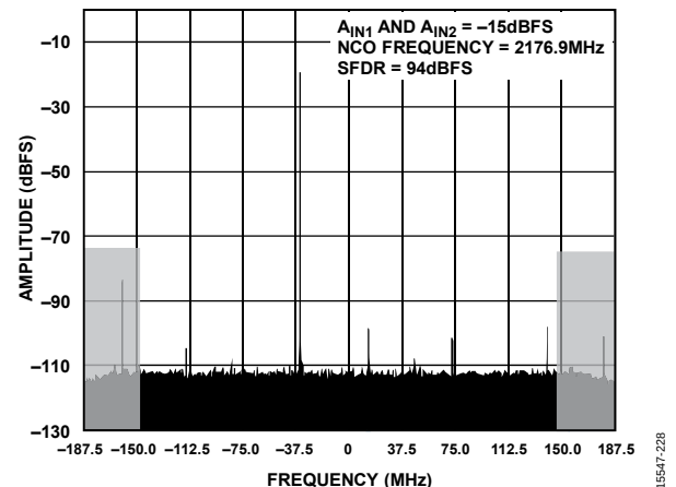
Figure 28. Two-Tone FFT; f_{IN1} = 1800 MHz, f_{IN2} = 2100 MHz f_{CLK} = 2.94912 GHz; Decimation Ratio = 8, NCO Frequency = 2176.92 MHz
