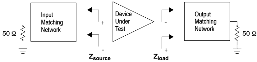
Figure 16. Series Equivalent 87.5-108 MHz FM Broadcast Reference Circuit Source and Load Impedance
