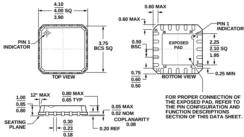
COMPLIANT TO JEDEC STANDARDS MO-220-VGGD-1 Figure 26. 20-Lead Lead Frame Chip Scale Package [LFCSP_VQ] 4 mm x 4 mm Body, Very Thin Quad (CP-20-1) Dimensions shown in millimeters
