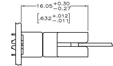
VERTICAL RECEPTACLE ASSEMBLY MATED TO VERTICAL PLUG STRADDLE ASSEMBLY
