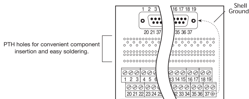
Female Connector SD-F37 37 Pin Socket Female Connector Shown with component counting holes (pads are on solder side)
