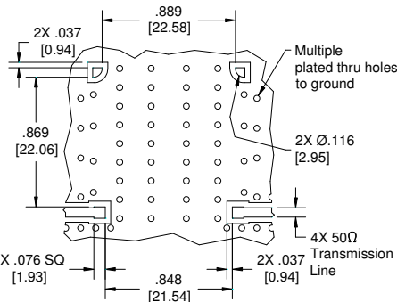
Dimensions are in Inches [Millimeters] XDL21-7-110 Rev B Mounting Footprint
