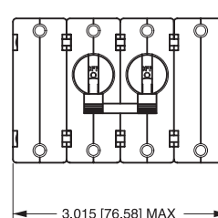
4-POLE (BB4)
