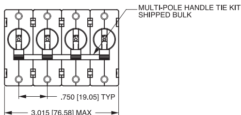
4-POLE (BB4)
