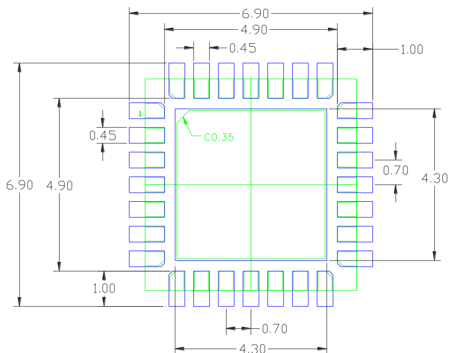
Figure 59. Recommended Land Pattern
