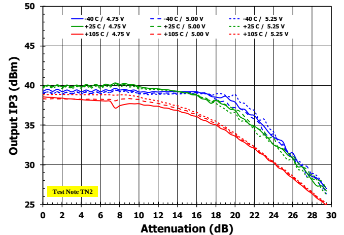
Figure 26. Output IP3 vs. Atten over Temp and Voltage [2.10 GHz]
