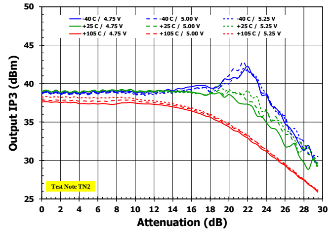
Figure 24. Output IP3 vs. Atten over Temp and Voltage [1.88 GHz]
