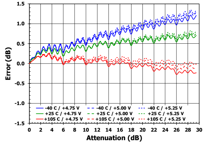
Figure 14. Step Accuracy vs. Atten over Temp and Voltage [1.88 GHz]
