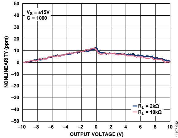
Figure 39. Gain Nonlinearity (G = 1000)
