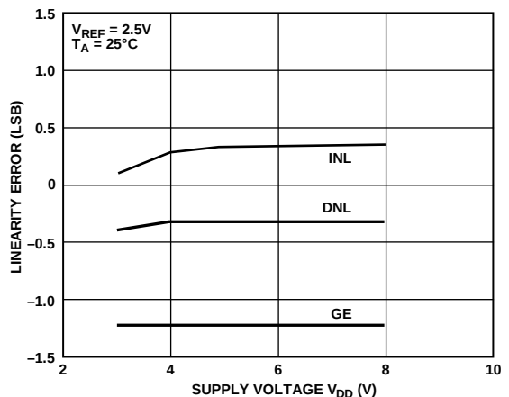
Figure 11. Linearity Error vs. V_{DD}
