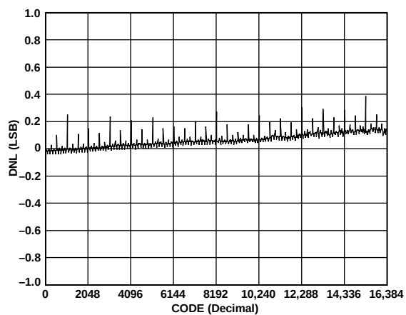
Figure 10. AD5553 DNL Error
