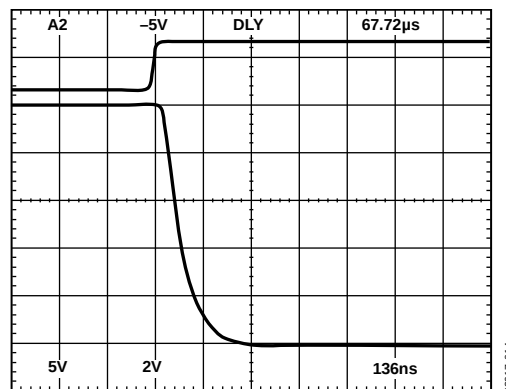
Figure 16. Settling Time
