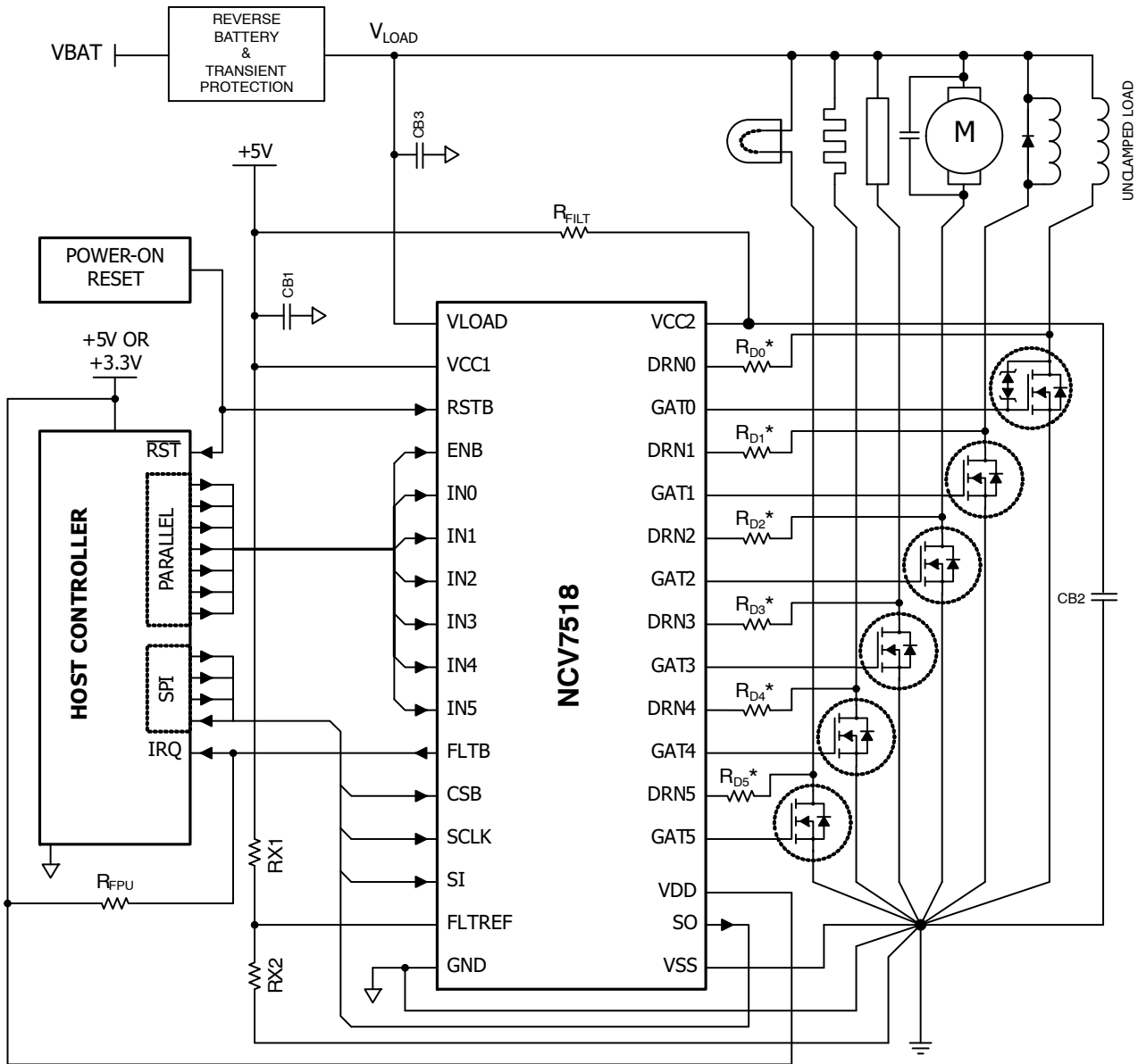
Figure 2. Application Diagram
