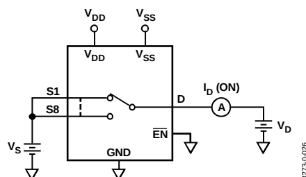
Figure 24. I_D (ON)
