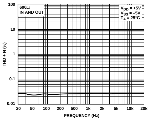
Figure 18. THD + Noise
