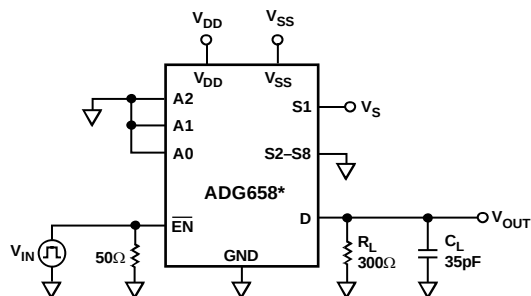
Figure 27. Enable Delay, t_{ON}(\overline{EN}) , t_{OFF}(\overline{EN})
