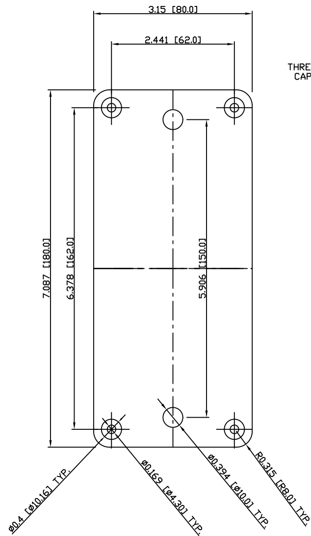
BOTTOM VIEW
