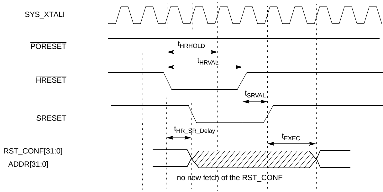
Figure 6. HRESET Behavior
