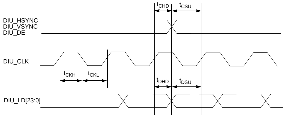
Figure 45. LCD Interface Timing Diagram – Access Level
