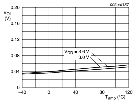
Fig 29. \overline{\text{EVENT}} output V_{OL} at I_{OL} = 2.1 mA
