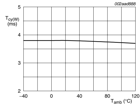
Fig 33. EEPROM write cycle time
