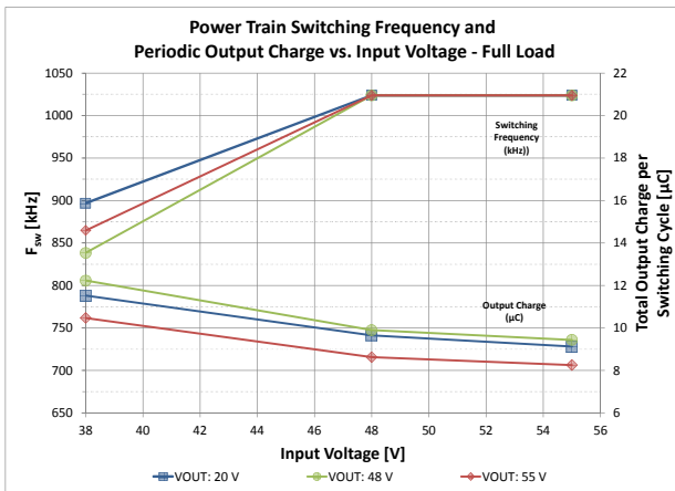
Figure 15: Power Train Switching Frequency and Periodic Output Charge vs. V_{\text{IN}} , V_{\text{OUT}} ; I_{\text{OUT}} = 10.42 \text{ A}
