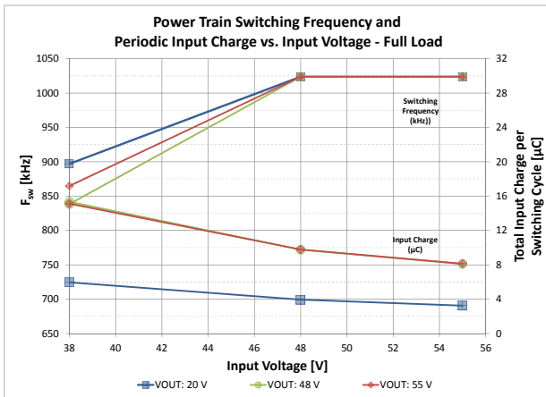
Figure 14: Power Train Switching Frequency and Periodic Input Charge vs. V_{\text{IN}} , V_{\text{OUT}} ; I_{\text{OUT}} = 10.42 \text{ A}
