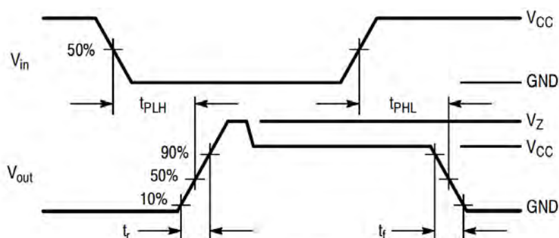
Figure 1. Switching Waveforms
