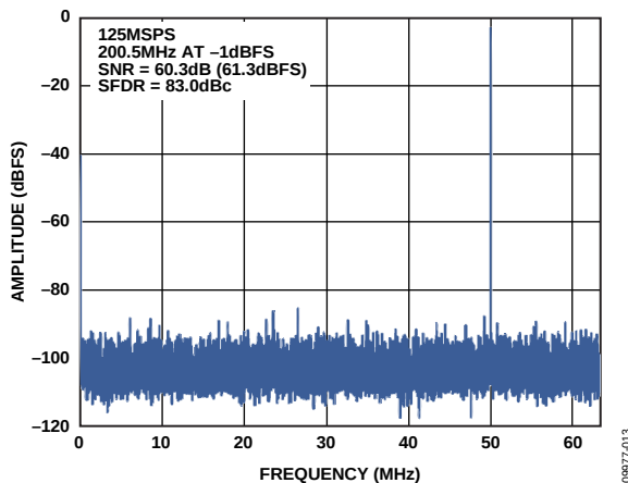
Figure 13. Single-Tone FFT with f_{IN} = 200.5 MHz
