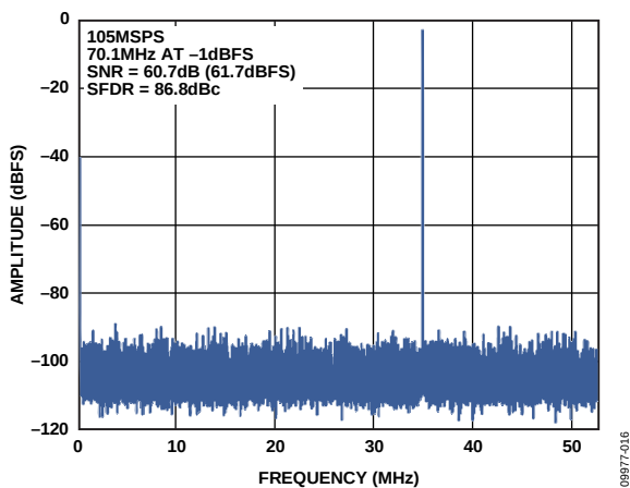
Figure 25. Single-Tone FFT with f_{IN} = 70.1 MHz
