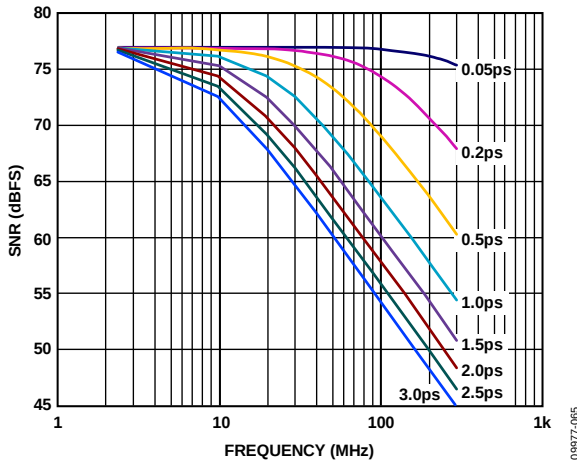
Figure 58. SNR vs. Input Frequency and Jitter
