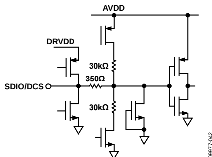
Figure 37. Equivalent SDIO/DCS Input Circuit
