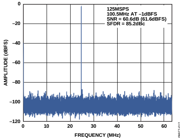
Figure 12. Single-Tone FFT with f_{IN} = 100.5 MHz
