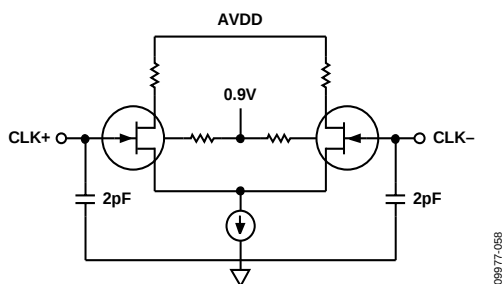
Figure 51. Equivalent Clock Input Circuit
