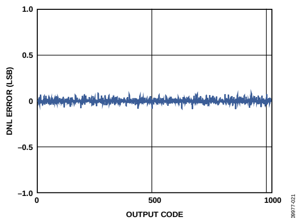
Figure 20. DNL Error with f_{IN} = 9.7 MHz
