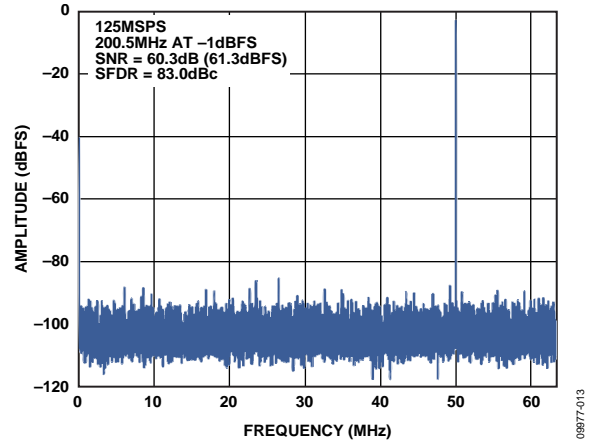
Figure 13. Single-Tone FFT with f_{IN} = 200.5 MHz
