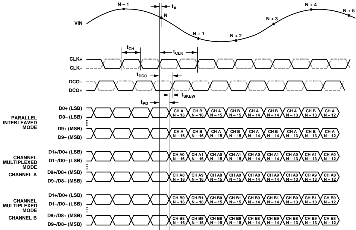
Figure 4. LVDS Modes for Data Output Timing
