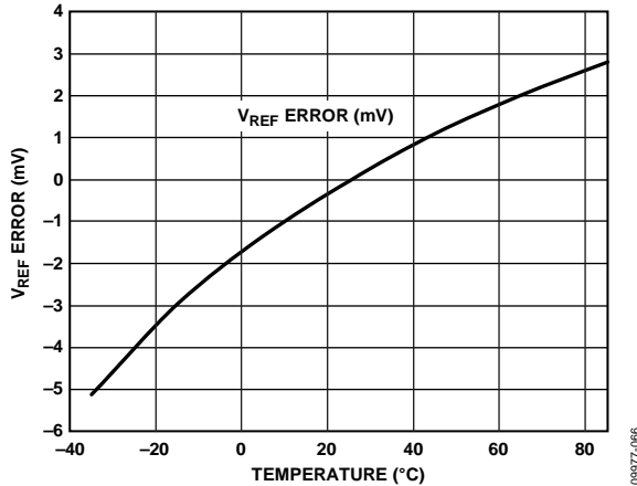
Figure 50. Typical V_{REF} Drift
