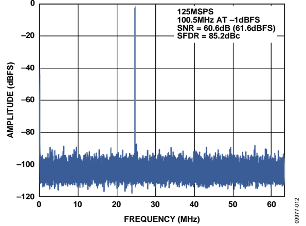
Figure 12. Single-Tone FFT with f_{IN} = 100.5 MHz
