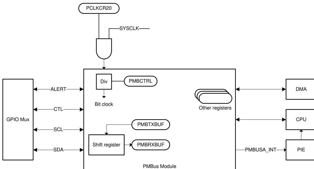
Figure 5-72. PMBus Block Diagram
