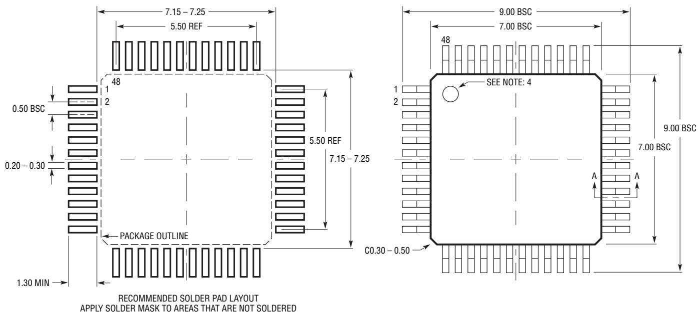
LX Package 48-Lead Plastic LQFP (7mm × 7mm) (Reference LTC DWG # 05-08-1760 Rev Ø)
