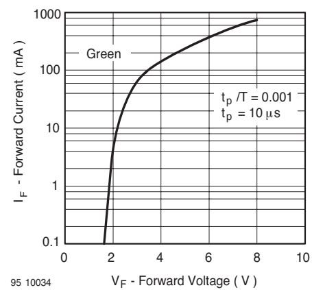
Figure 20. Forward Current vs. Forward Voltage
