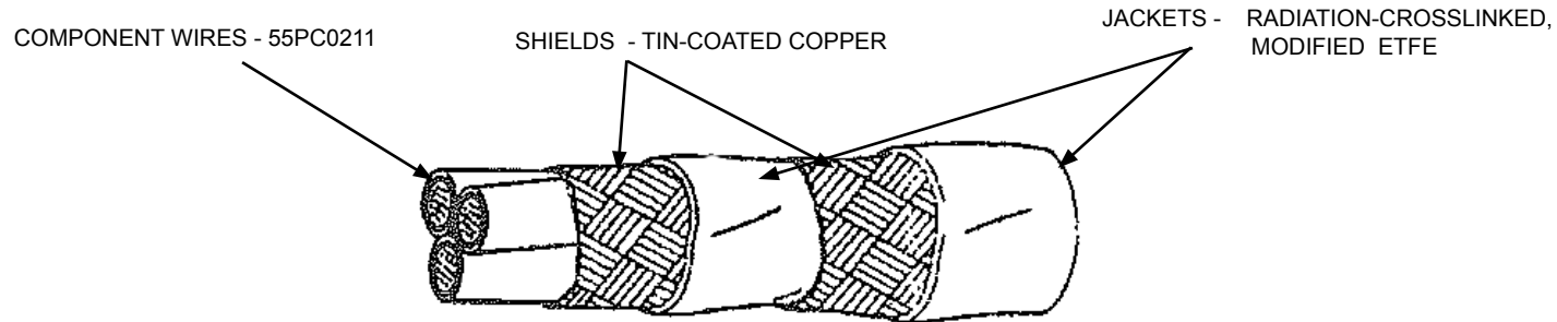
CABLE CONSTRUCTION DETAILS
