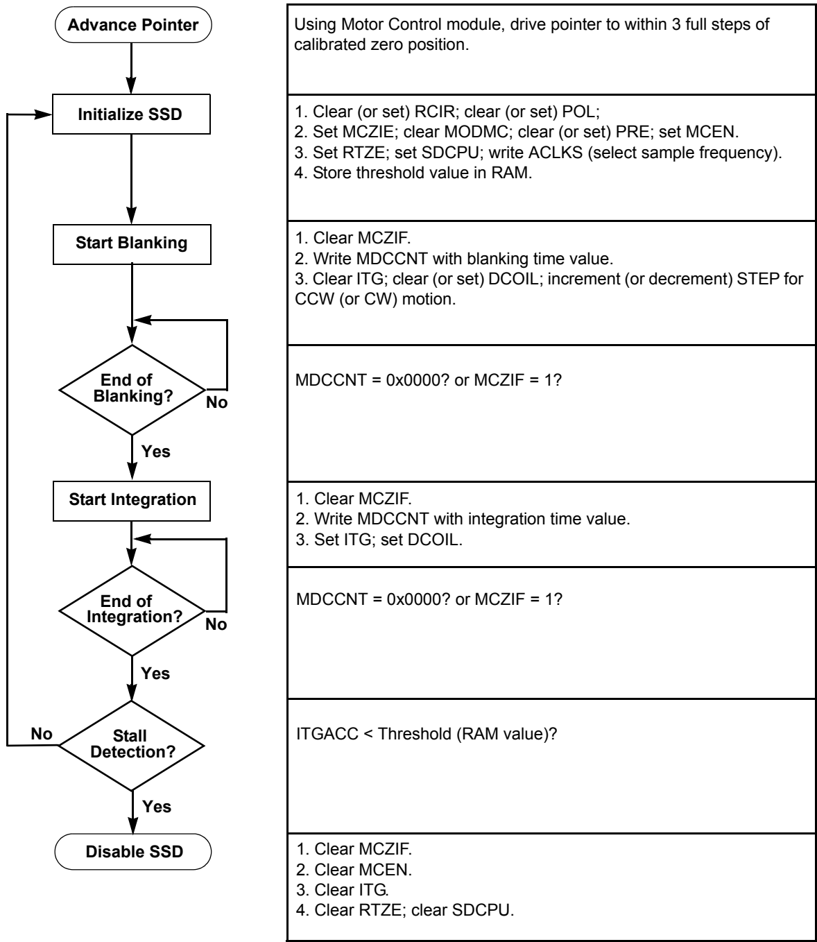
Figure 17-15. Return-to-Zero Flowchart
