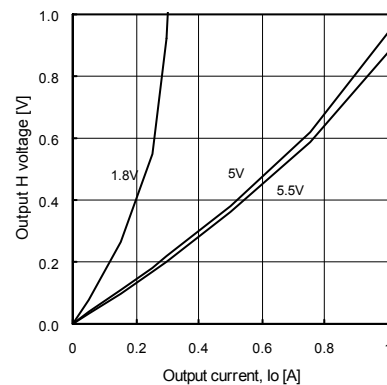
Fig.6 Output H voltage (Voltage characteristics)
