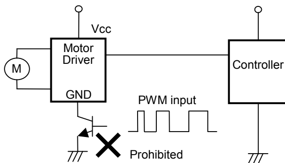
Fig.22 GND Line PWM switching prohibited
