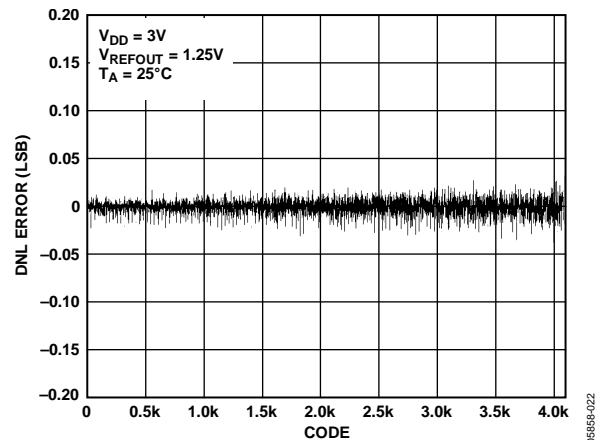
Figure 21. DNL—AD5623R-3
