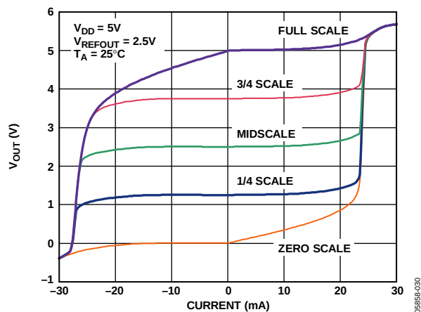
Figure 32. AD5623R-5/AD5643R-5/AD5663R-5 Source and Sink Capability
