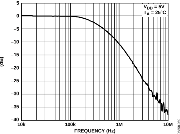
Figure 47. Multiplying Bandwidth
